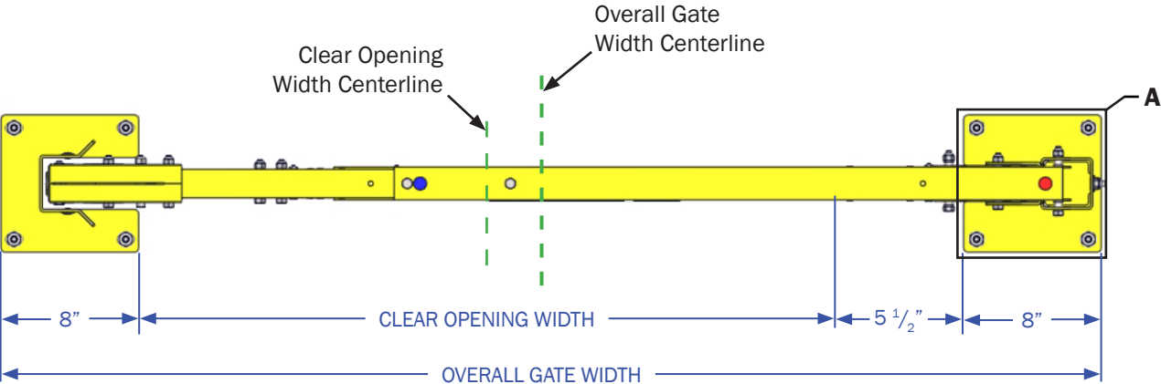
TOP VIEW
